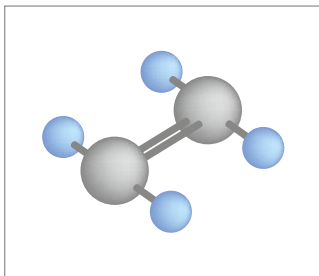
Abb. 5-1 Ethylen
